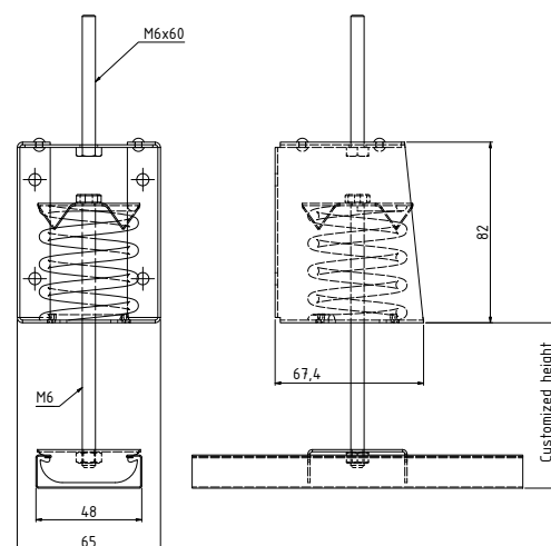
VT-MSH Top-mounted With click-on system
